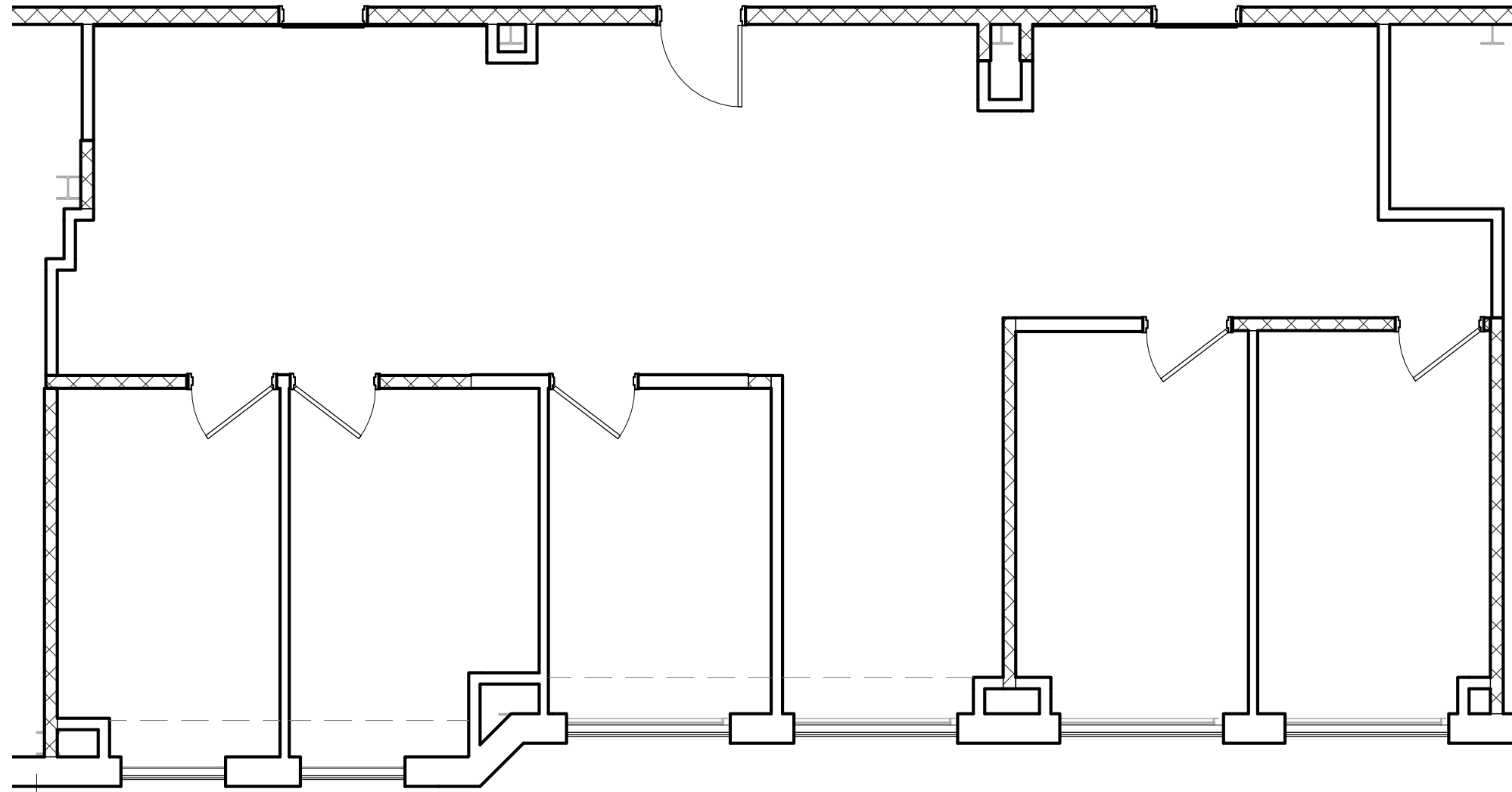
1 EXISTING SUITE 1009 3/16" = 1'-0"
