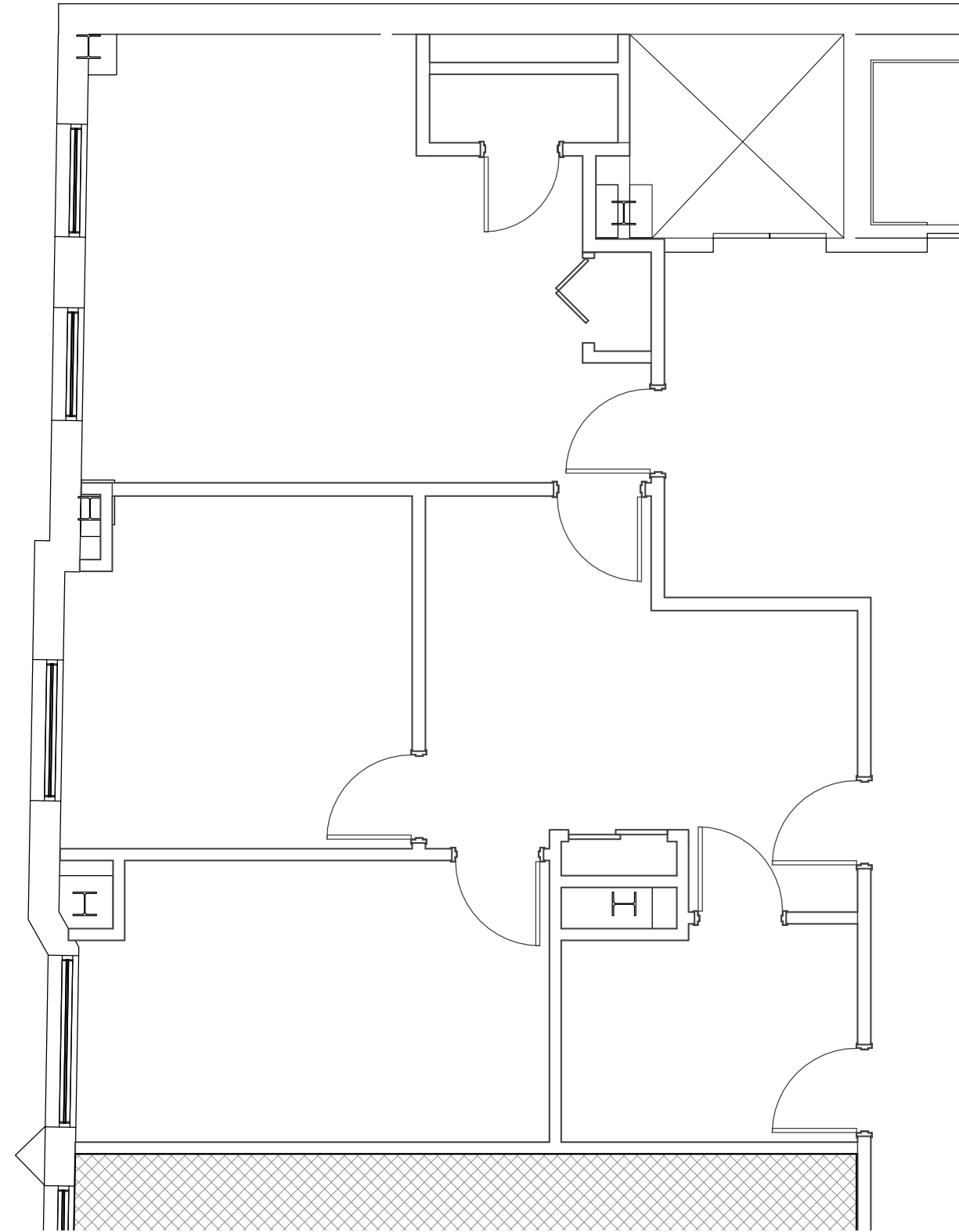
1 EXISTING CONDITIONS PLAN 3/16" = 1'-0"
