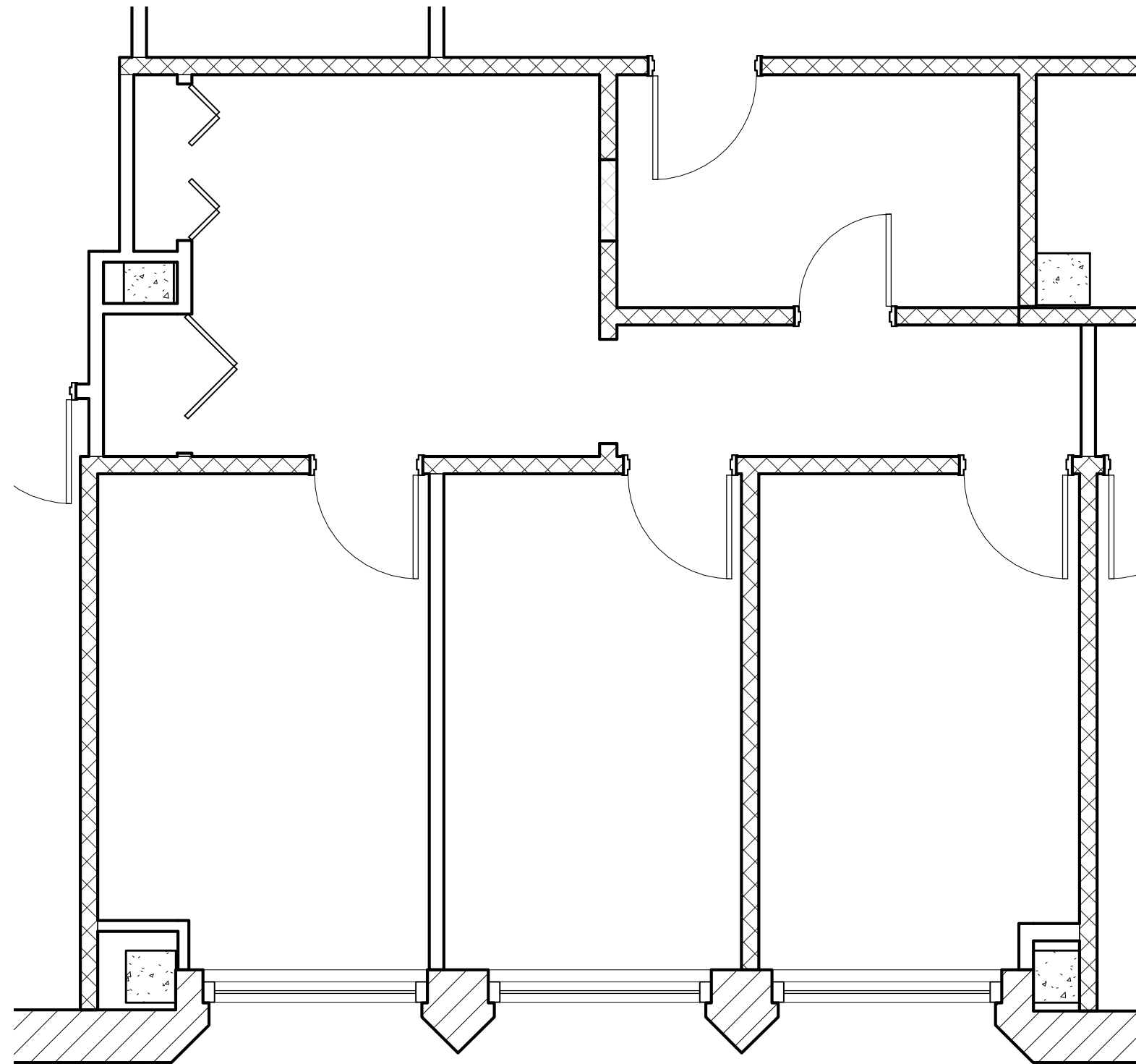
1 EXISTING FLOOR PLAN 1/4" = 1'-0"
